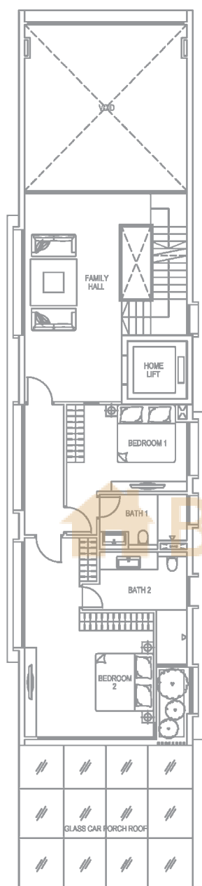
2ND STOREY
