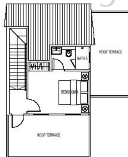
ATTIC PLAN
