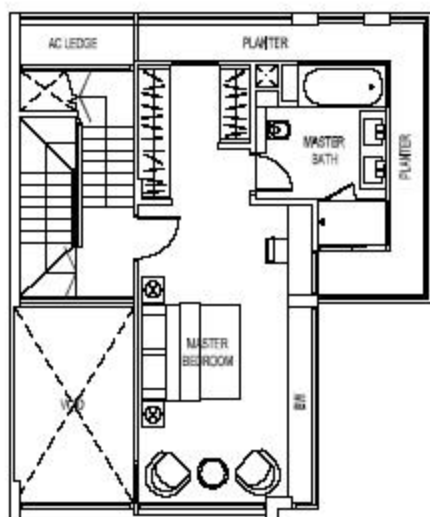
2ND STOREY PLAN
