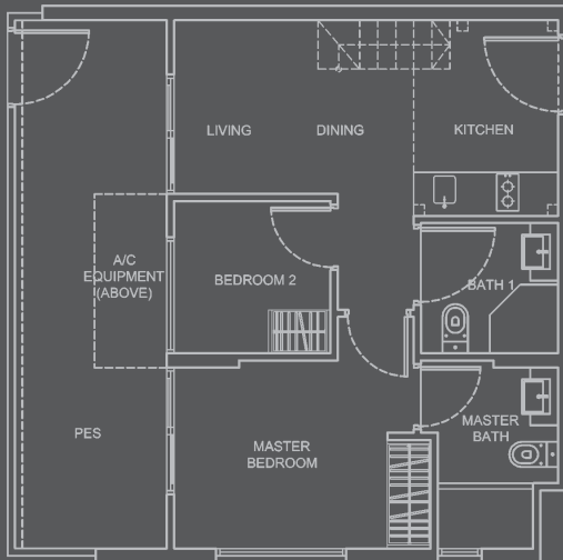
Type A3-G1 (High Ceiling) #01-21 Area 58 sqm
