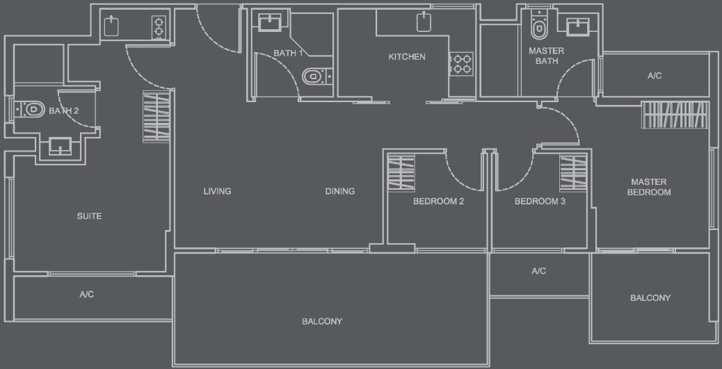
Type D3-T #02-11 to #04-11 Area 111 sqm
