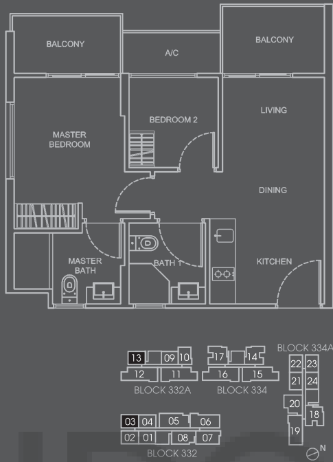
Type A1-T #02-03 to #04-03, #02-13 to #04-13 Area 50 sqm
