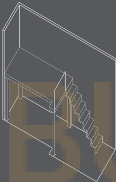
LOFT LAYOUT (Isometric View)
