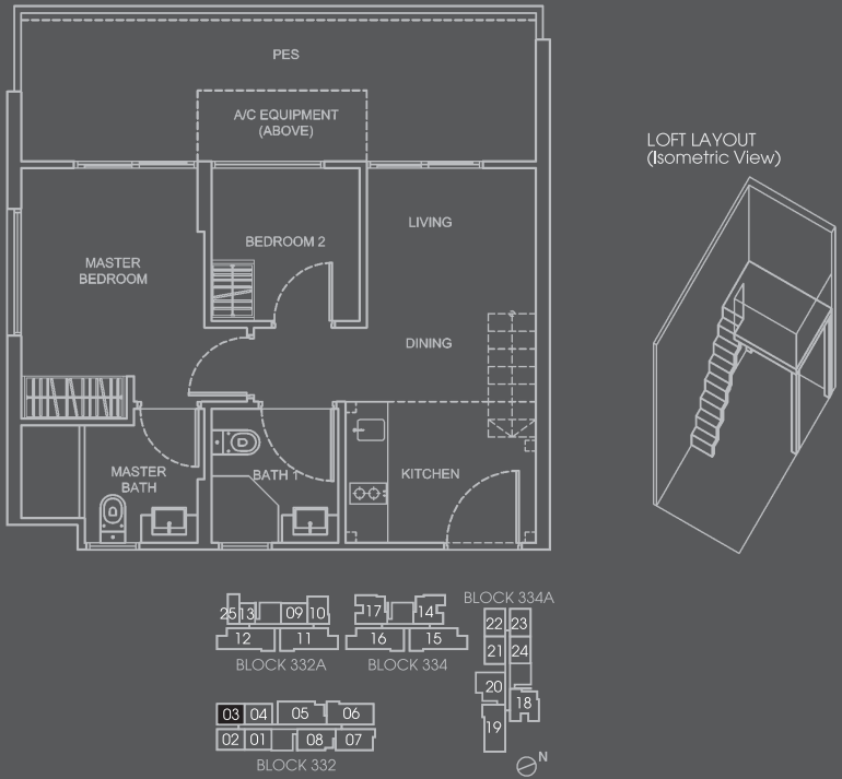
Type A1-G (High Ceiling) #01-03 Area 57 sqm
