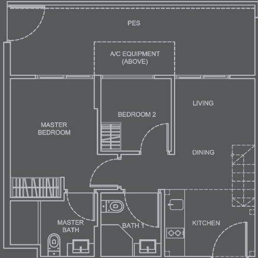
Type A4-G1 (High Ceiling) #01-09 Area 59 sqm
