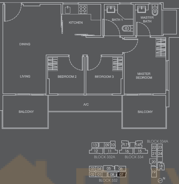
Type B3-T #02-07 to #04-07 Area 72 sqm
