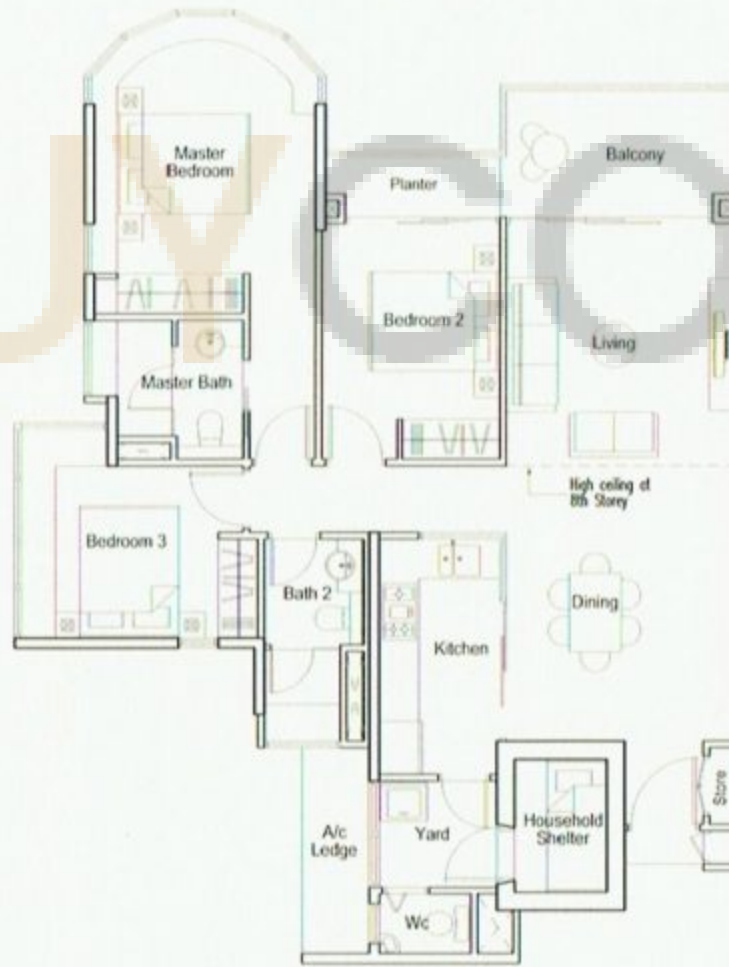
TYPE C3(a) ■ 114sqm/1227sqft
