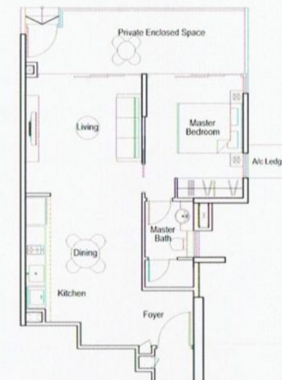
TYPE A2 (a)p ■ 64sqm/689sqft
