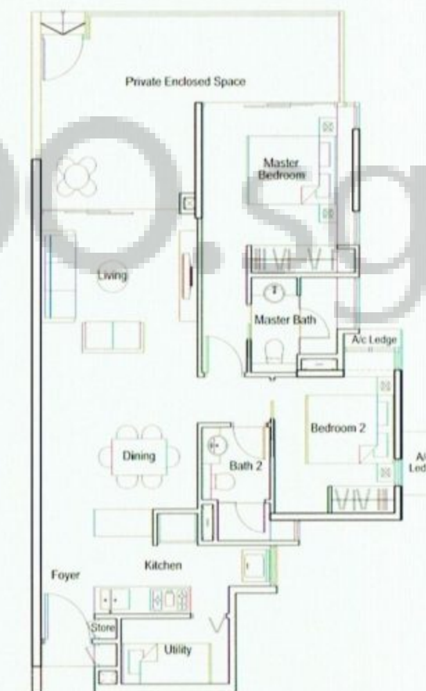
TYPE B3p 100sqm/1076sqft
