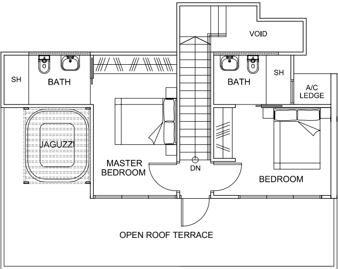
ATTIC PLAN
