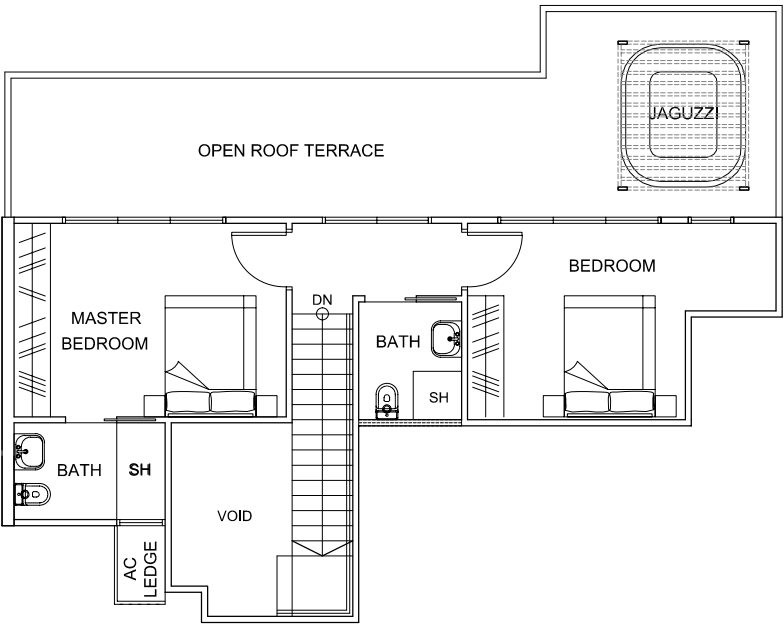
ATTIC PLAN
