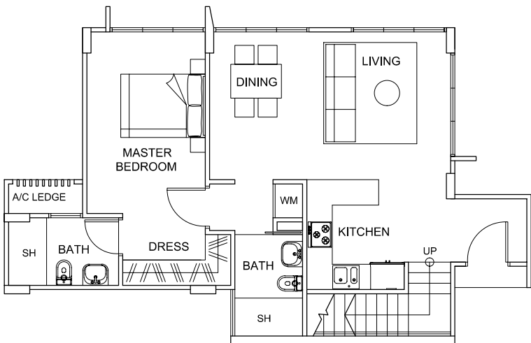
5TH STOREY PLAN
