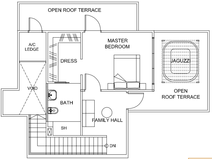
ATTIC PLAN
