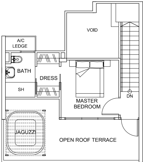
ATTIC PLAN
