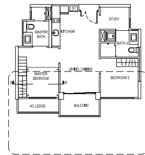
TYPE SB4a 63 sq m / 678 sq ft #02-19 to #20-19
