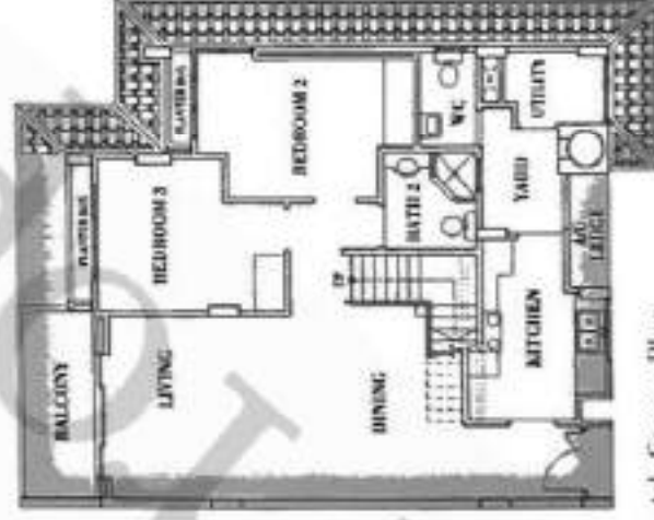
Type D6 (b) Floor Area: 139 sqm/1496 sq ft
