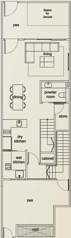
1st STOREY
