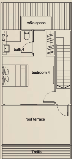
ATTIC
