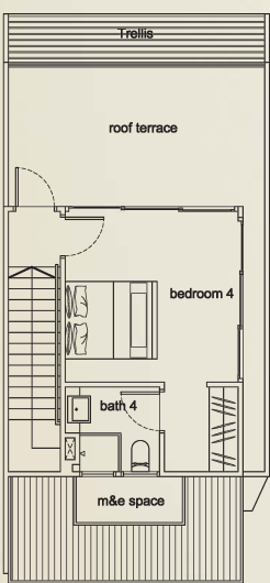
ATTIC
