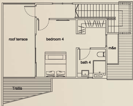
ATTIC
