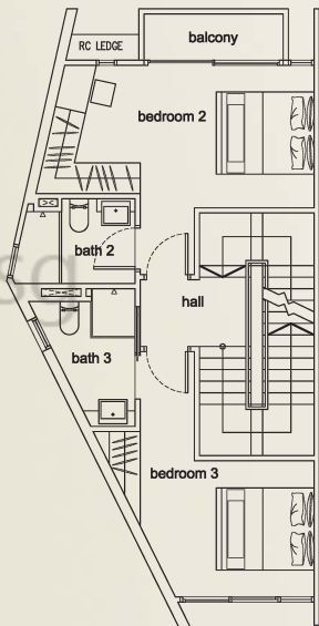
3rd STOREY
