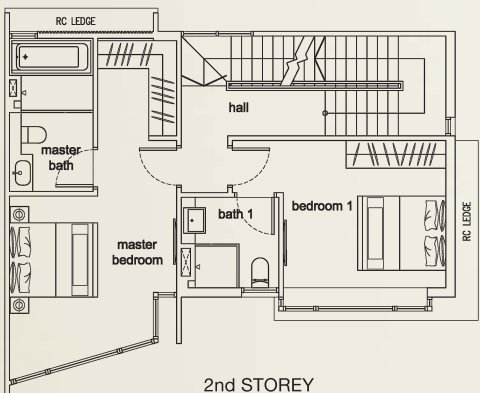
2nd STOREY
