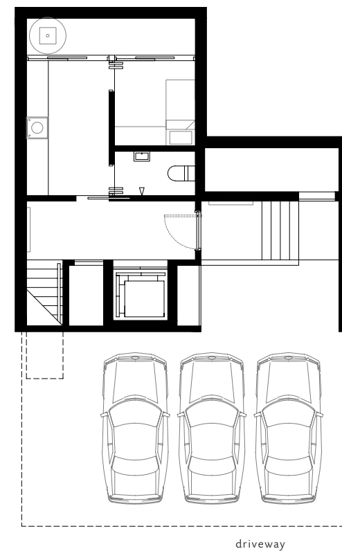
BASEMENT
