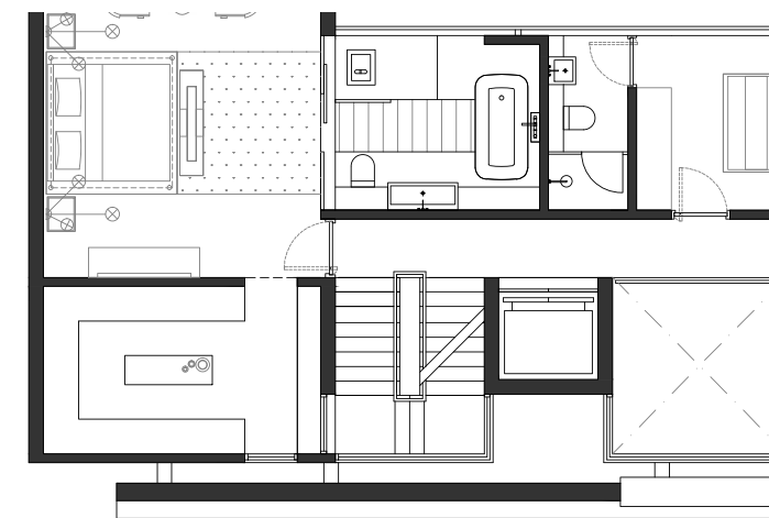
2ND FLOOR
