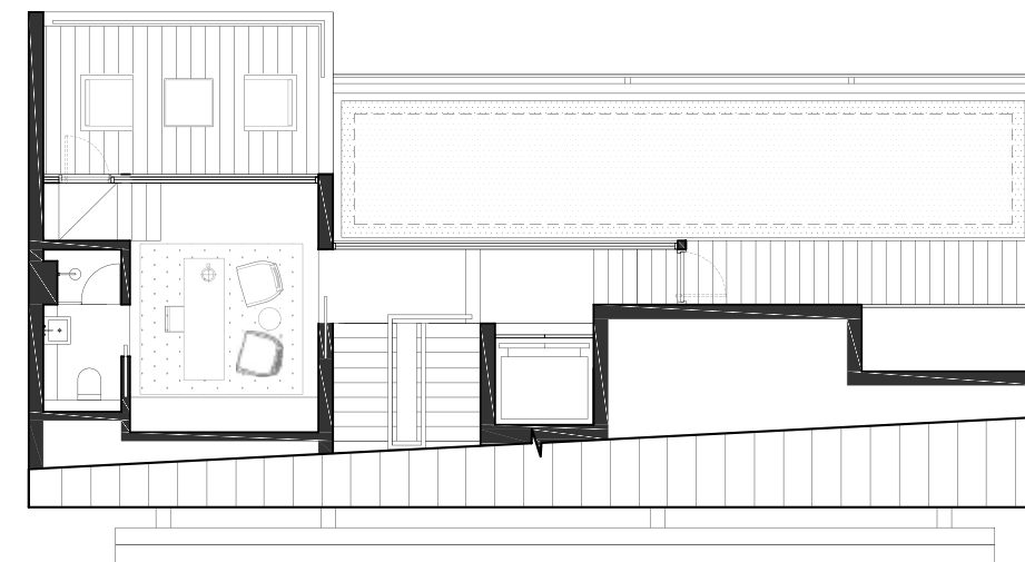
2ND FLOOR
