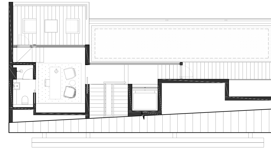
ATTIC
