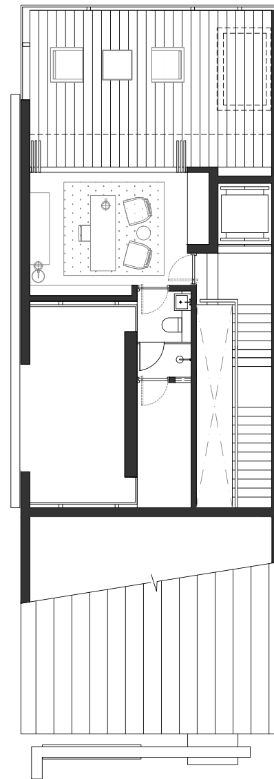
ATTIC
