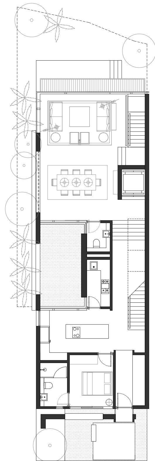
1ST FLOOR
