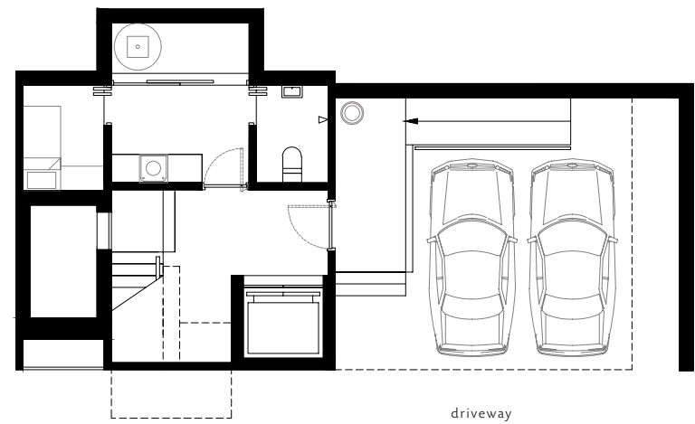
BASEMENT
