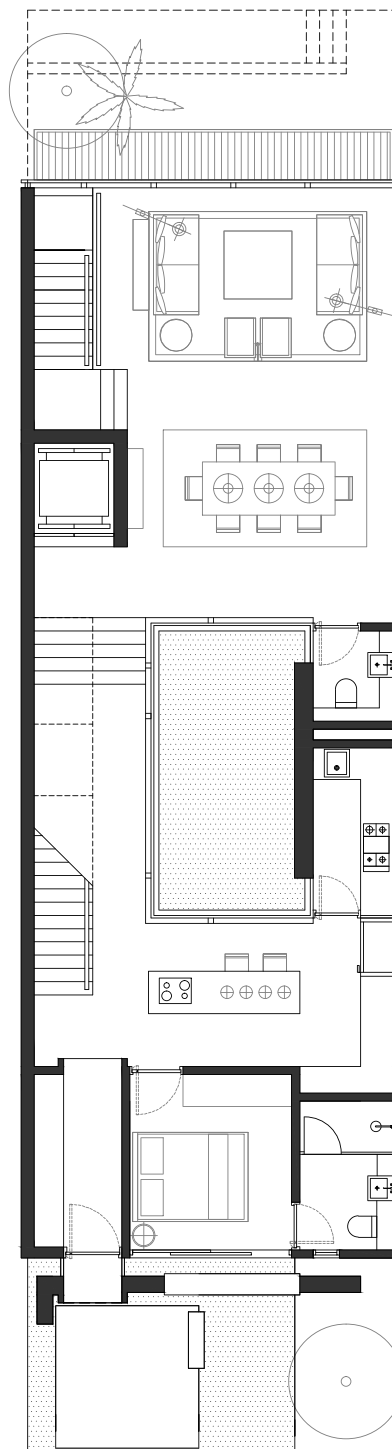
1ST FLOOR
