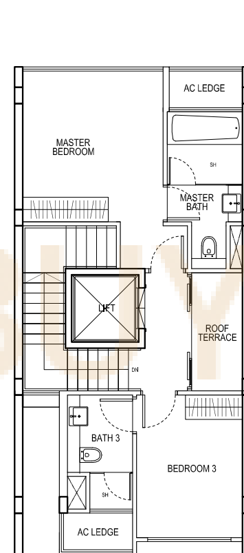
THIRD STOREY LEVEL
