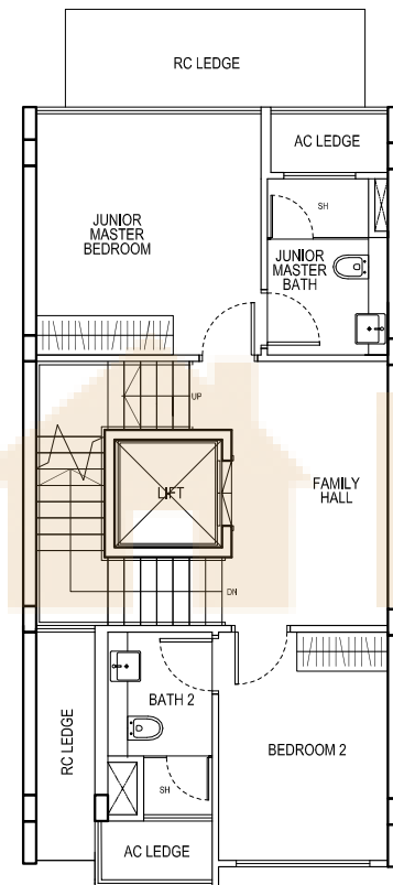
SECOND STOREY LEVEL
